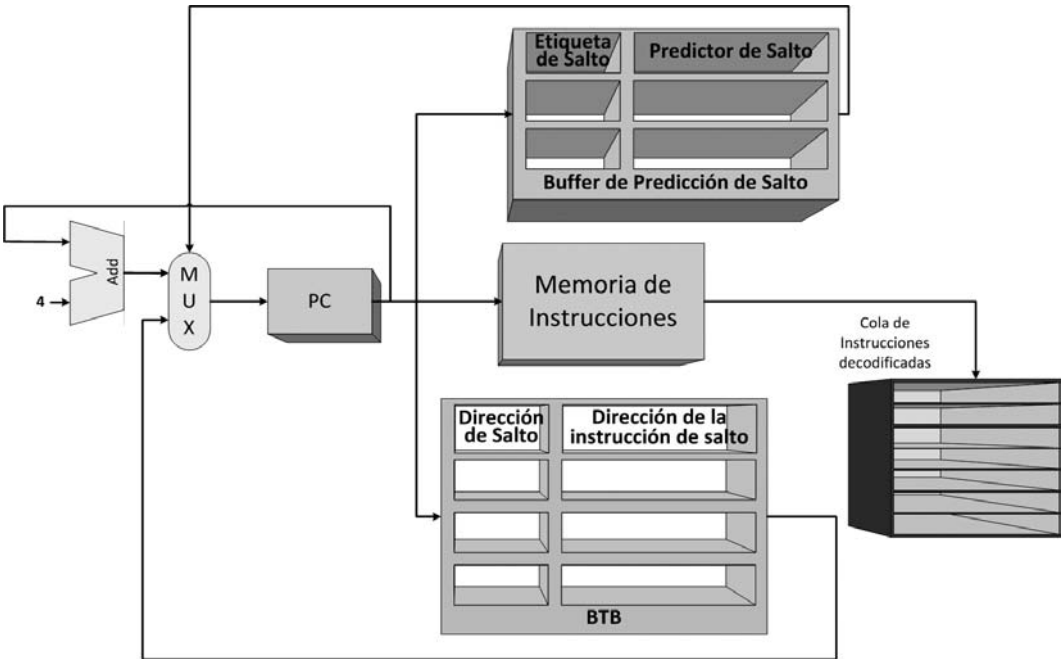
BTB (Branch Target Buffer).
